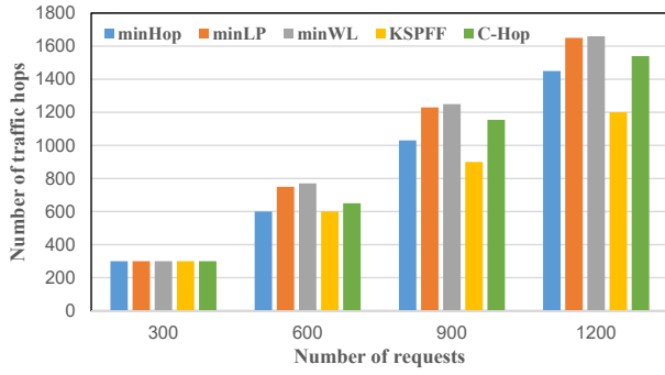
Fig. 6: The number of traffic hops vs the number of network slice requests.
