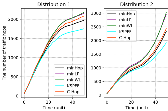
Fig. 11: The number of traffic hops for two slice arrival distributions over time.
